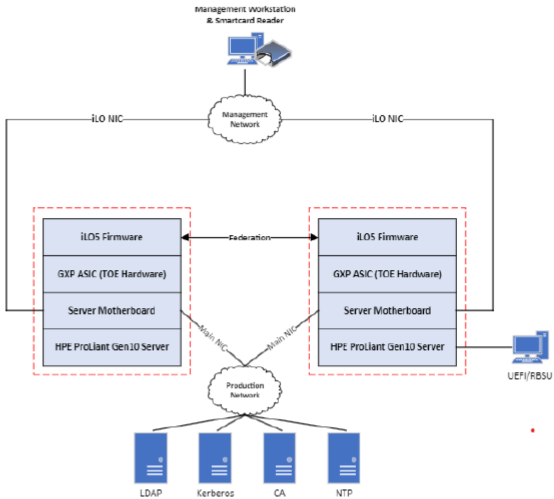
Figure 1: TOE Architecture
